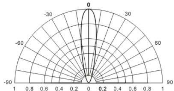
Beam Pattern
