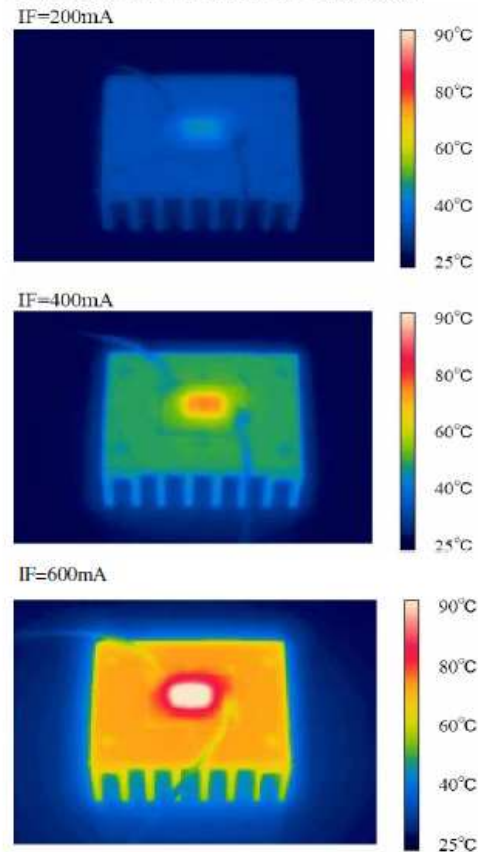
<Fig.2> Board A (surface area=10,300mm 2 )
